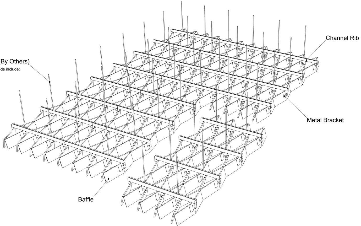
⑤ PERSPECTIVE VIEW
