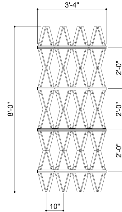
③ PLAN VIEW MODULAR TYP
