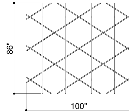
② BOTTOM FACE VIEW
