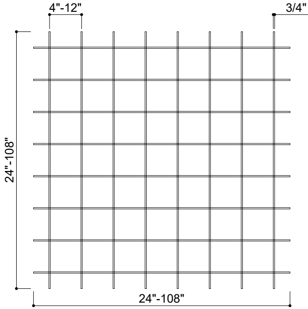
① PLAN VIEW
