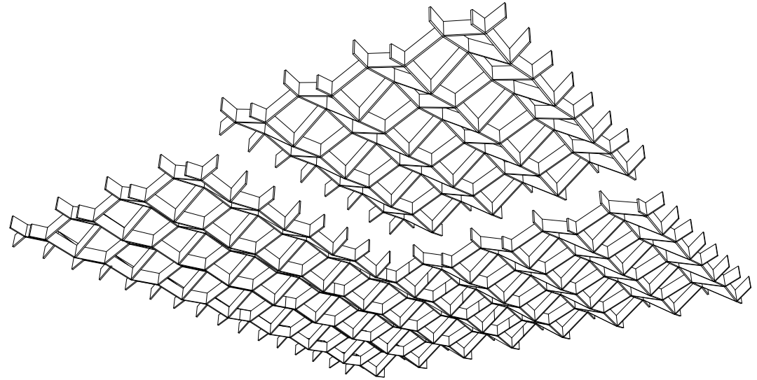
② PERSPECTIVE VIEW
