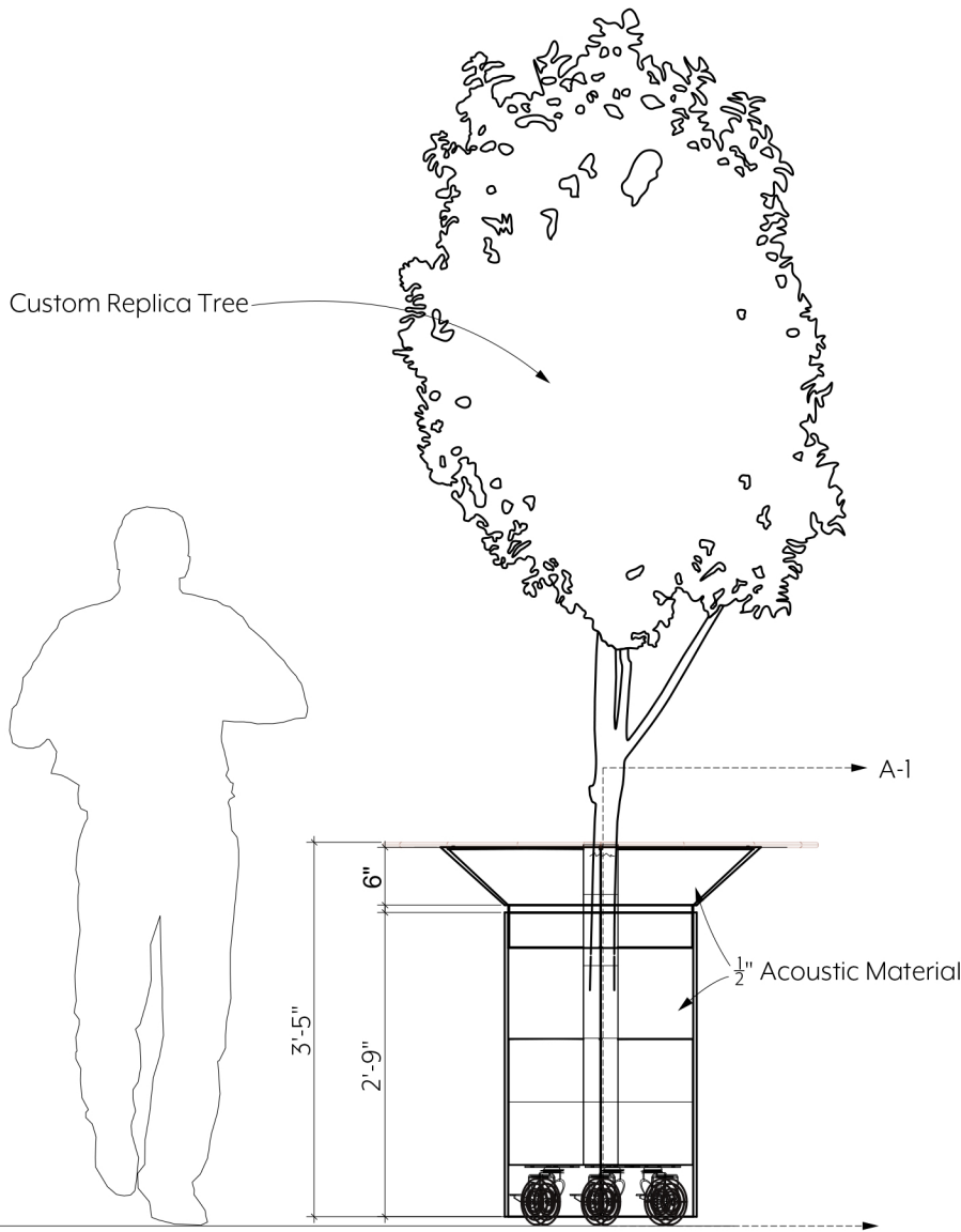
1 FRONT VIEW
