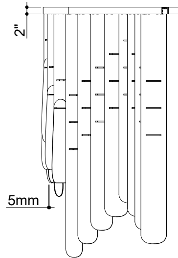
② SIDE VIEW
