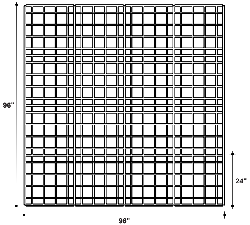
① BOTTOM VIEW
